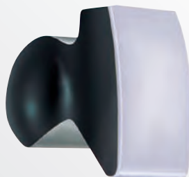
11 Universal Dollies faces 75 x 55 mm and 60 x 45 mm, height 57 mm, 1100 g Art.No. 2002010000
