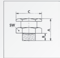
6 T1/B Button Head Grease Nipples hexagonal head, hexagon version, galvanized C: Ø 16 mm, SW: 15 mm
