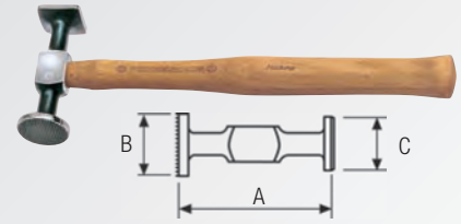
3 Bumping Hammers short execution, round face chequered
