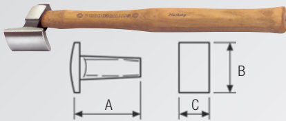
7 Single End Planishing Hammers with bowed face
