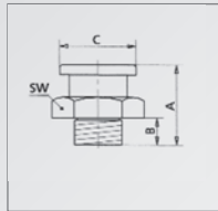
5 M1 Button Head Grease Nipples round head, hexagon version, galvanized C: Ø 16 mm, SW: 17 mm
