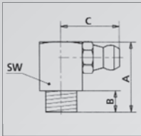
4 Type H3 VK square version - 90° angled, galvanized
