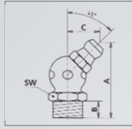
2 Type H2 SK hexagon version - 45° angled, galvanized
