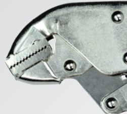
4 Parallel Grips with drop-forged chrome vanadium steel jaws; used for flat and shaped materials
